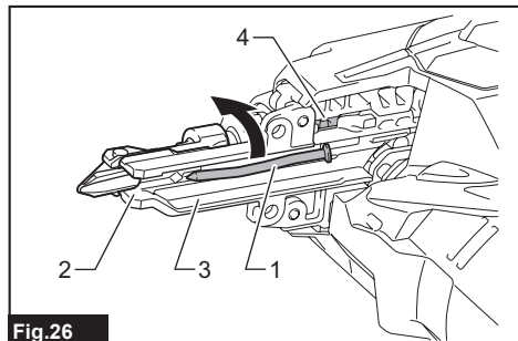
Fig. 26 ► 1. Jammed fastener 2. Fastener exit opening 3. Driver guide 4. Lock groove
